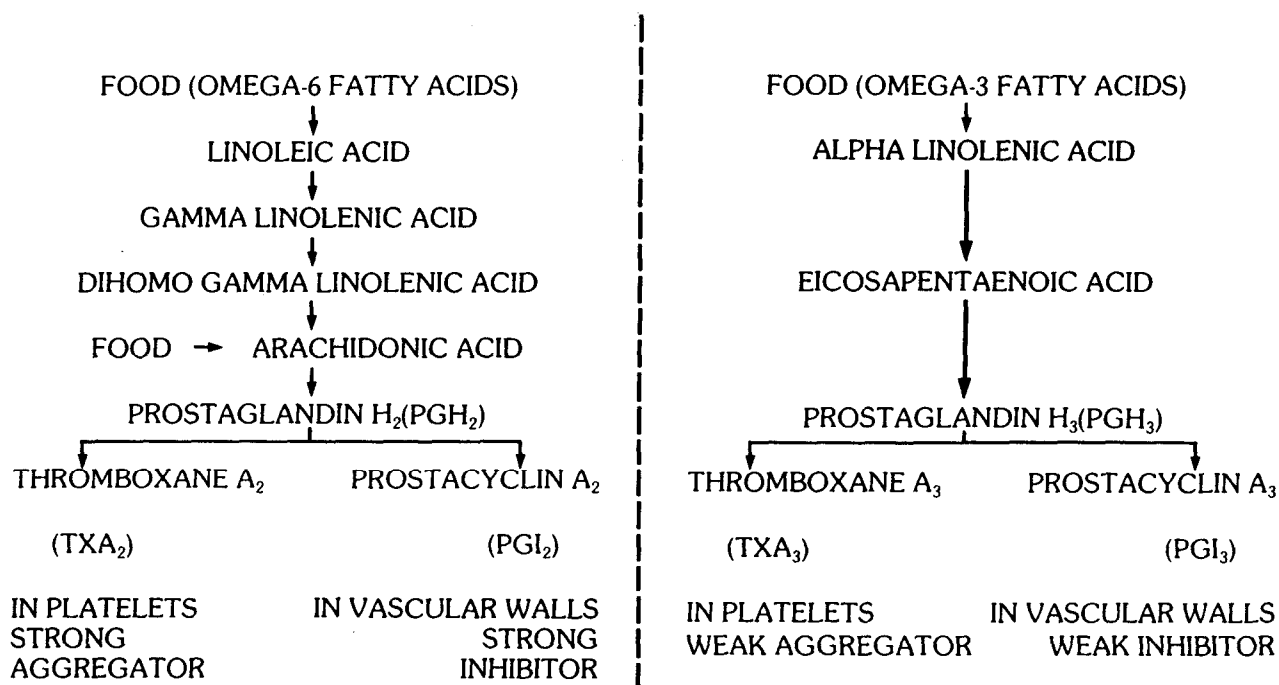
Figure 1. Synthesis of platelet aggregatory and anti-aggregatory biochemicals. 186
